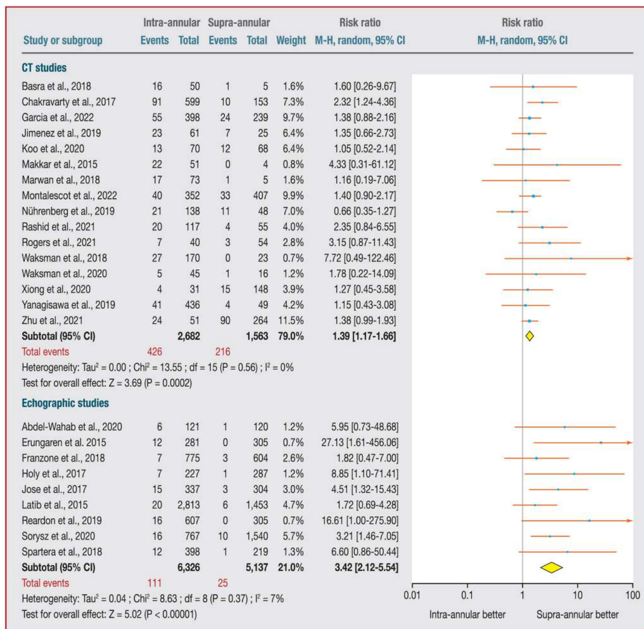
Fig. 3. Forest plot of selected studies comparing the effect of intra-annular versus supra-annular transcatheter aortic valve replacement on the occurrence of leaflet thrombosis.
